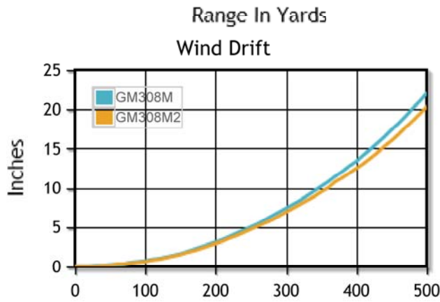
Range In Yards Wind Drift in Inches (at 10 MPH Crosswind)
