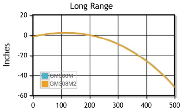
Range In Yards Trajectory for a 200 yards zero with a sight height of 1.5 inches.
